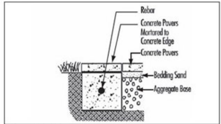
Figure 10. Submerged concrete edge.
